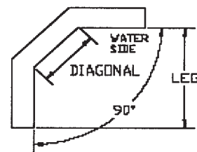
90° Diagonal Double Weld
