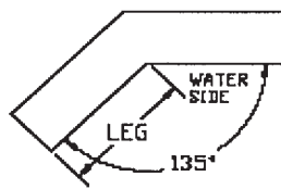
135° Single Weld
