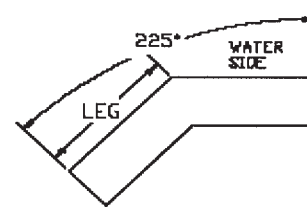
225° Single Weld
