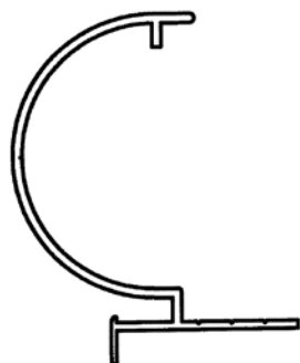
CP-2 Bullnose Liner Track with Alignment Edge 2.38" Top of Coping to Mounting Surface 1.62" Mounting Surface Width
