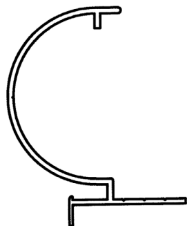
CP-2P Bullnose Liner Track with Alignment Edge 2.38" Top of Coping to Mounting Surface 2" Mounting Surface Width
